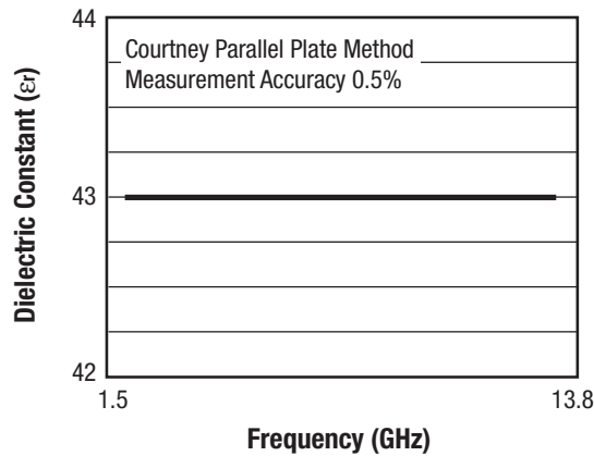
Figure 3. Typical (εr) vs Frequency
